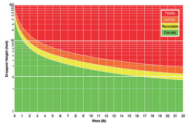
Above: Common dropped objects (first). Typical loose fixing (second). DROPS calculator (third).
